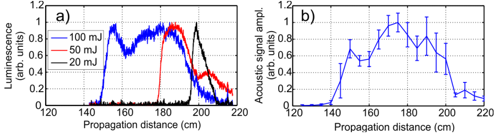
Fig. 2. Luminescence power (a) and acoustic signal amplitude (b) recorded for beam focused with 2 m focal length lens. Acoustic signal amplitude was recorded for 100 mJ energy pulse and with a repetition rate of 1 kHz.
