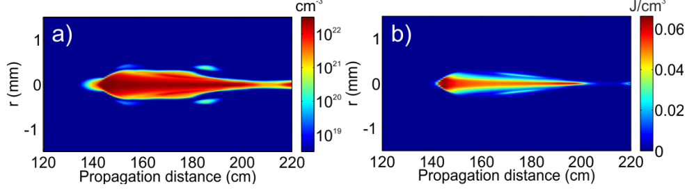
Fig. 9. Energy deposition and plasma density dependence on propagation distance for a 100 mJ energy pulse focused by 2 m focal length lens.
