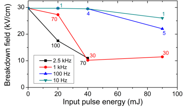
Fig. 11. Breakdown field dependence on laser pulse energy measured for different repetition rates. For each measurement the average number of laser shots necessary to obtain the breakdown is also indicated.
