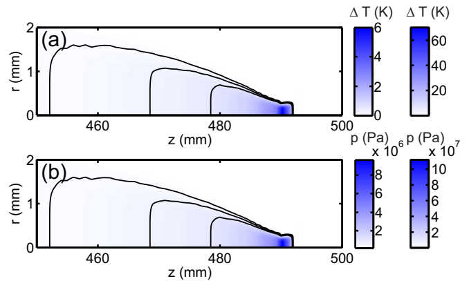
FIG. 9. Initial (a) temperature and (b) pressure distributions for peak heatings of \Delta T_{max} \equiv \max\{T(r, z, t = 0) - T_0\} = 6 K (leftmost colorbars) and \Delta T_{max} = 70 K (rightmost colorbars). The contours are at 1/10, 1/20, and 1/50 of the difference between the maximum and background levels, p_0 = 1.023 \times 10^5 Pa (corresponding to a depth of the order of 10 cm in water of background density \rho_0 = 998.2 \text{ kg}/\text{m}^3 ), and T_0 = 300 K. Same criterion for contours is applied to Figs. 10 and 11.
