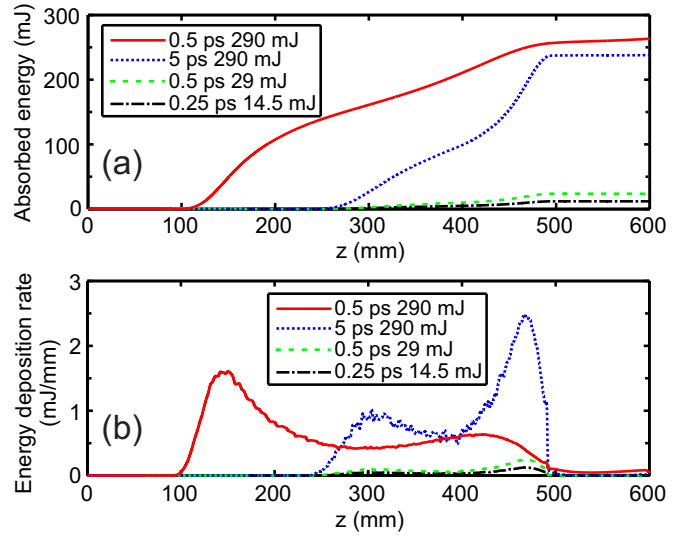
FIG. 6. (a) Absorbed energy, \langle U \rangle , and (b) rate of nonlinear energy losses, d\langle U \rangle/dz , as a function of propagation distance. The curves correspond to different input pulse energies and pulse durations: 290 mJ, 5 ps (dotted blue); 290 mJ, 0.5 ps (solid red), 29 mJ, 0.5 ps (dashed green) and 14.5 mJ, 0.25 ps (dash-dot black). The dotted blue and solid red curves correspond to pulses with the same energy while the dotted blue, dashed green and dash-dot black curves correspond to beams with the same peak power.
