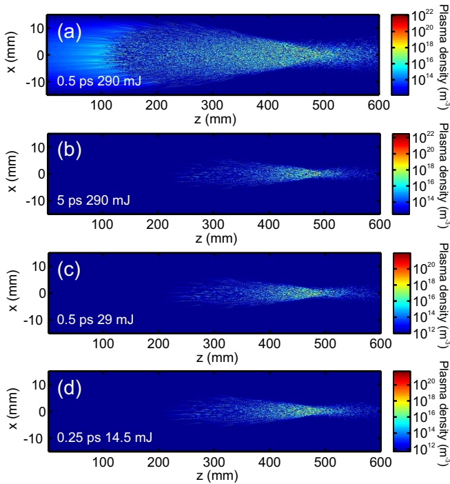
FIG. 5. Plasma density, \rho_e , profiles in the same conditions as in Fig. 4 is depicted in (a) and (b) i.e. when input pulse energy 290 mJ and pulse duration: (a) 0.5 ps; (b) 5 ps. While (b), (c) and (d) are for the cases when input beam peak power was the same for pulse durations 5, 0.5 and 0.25 ps respectively. Maximum plasma densities are 12.4 \times 10^{21} , 31 \times 10^{21} , 9.5 \times 10^{21} , 4.9 \times 10^{21} \text{ m}^{-3} for (a), (b), (c), (d) respectively.
