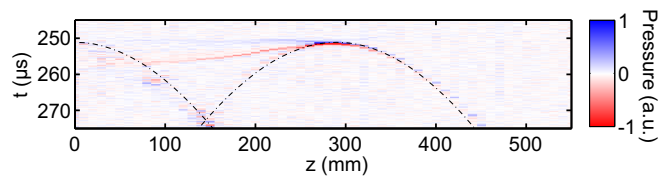
FIG. 2. Typical acoustic wave profile registered by a hydrophone. The focusing lens was 30 cm above the surface of water and the pulse duration was 5 ps. The two dashed curves represent the profiles of the two spherical acoustic waves emitted from point sources located at the depths z = 0 and 297 mm (corresponding to the position of the top of the hyperbolic branches). These locations clearly correspond to the water tank surface and to the laser focal region, respectively.
