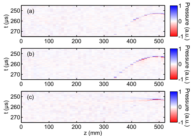
FIG. 3. Comparison of amplitude profiles for the acoustic waves generated by 290 mJ laser pulses with initial duration of (a) 0.25 ps, (b) 0.5 ps, and (c) 5 ps. The lens was positioned at h = 13 cm above the surface of water corresponding to a focus depth of z_0 \sim 500 mm. Acoustic waves are registered by moving the hydrophone along a vertical axis at distance d = 38 cm from the laser propagation axis.
