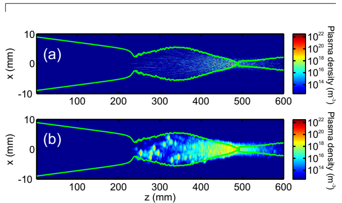
FIG. 7. Plasma density, \rho_e , distribution from the simulation of pulse propagation with initial energy of 290 mJ and duration of 5 ps (a). The solid green curve represents the boundary of the focal (plasma) volume. (b) Spectrally filtered plasma density distribution for the same conditions. A log scale is used for both figures.
