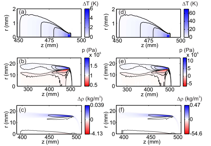
FIG. 10. (a,d) Temperature, \Delta T , (b,e) pressure, p , and (c,f) density \Delta \rho \equiv \rho - \rho_0 , distributions in water 10 \mu\text{s} after the pulse heating. (a-c) \Delta T_{max} = 6 \text{ K} , (d-f) \Delta T_{max} = 70 \text{ K} . \rho_0 = 998.2 \text{ kg/m}^3 and T_0 = 300 \text{ K} .
