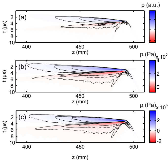
FIG. 11. Simulated pressure vs time signal recorded at an offset of 5 mm from the pulse propagation axis, z . Simulations show (a) linear (Eqns. 6) and (b,c) nonlinear (Eqns. 7) calculations, the latter for (b) \Delta T_{max} = 6 K and (c) \Delta T_{max} = 70 K.
