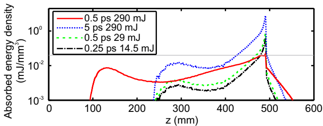
FIG. 8. Absorbed energy density, U_m , versus propagation distance. Different initial beam energies and pulse durations are represented with different colors and are the same as in Fig. 6. The thin gray horizontal line represents an approximate threshold value ( 40 \mu\text{J}/\text{mm}^3 ) for pressure wave to be registered by the hydrophone (see Fig. 1).
