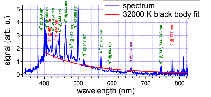
Figure 4. Time-integrated emission spectrum of the discharge plasma recorded for the 36 A current pulse, corrected for the spectral response of the optical system. Main emission lines are indicated on the graph: green for N^+ lines, red for O and O^+ lines and violet for H lines.
