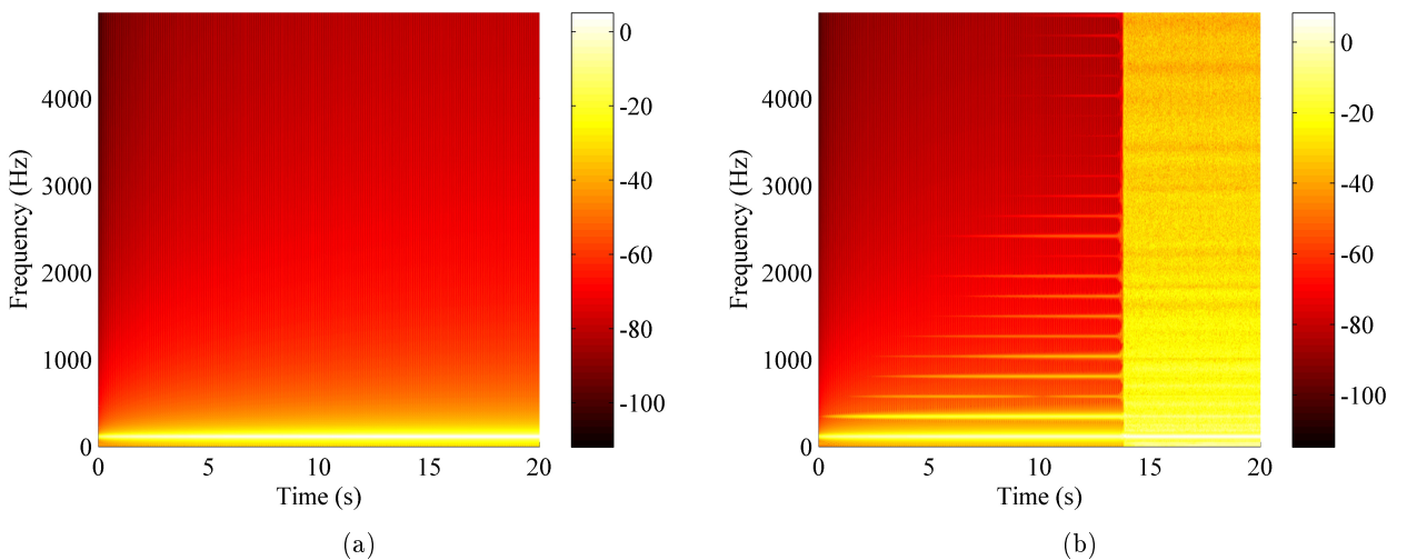
Figure 7: Spectrograms of output velocity at point (x_0=0.6 m, y_0=0.01 m) for a forcing at 115 Hz from 0 to 20 N in 20 s, for beams (a) U and (b) E0. Color scale in dB (ref. 1 \text{ m}\cdot\text{s}^{-1} )
