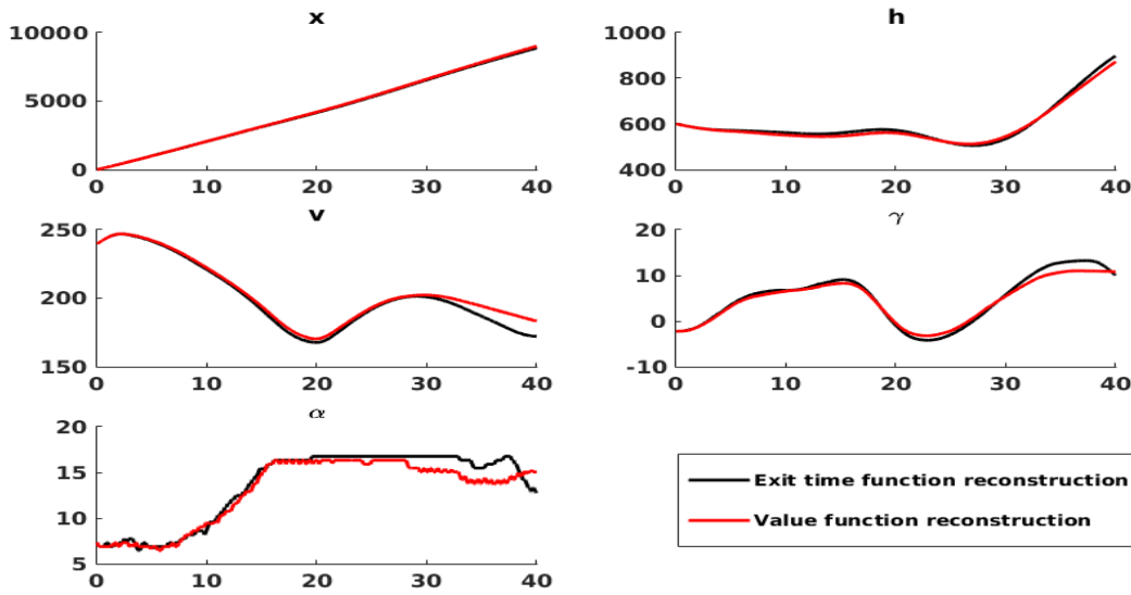
Figure 2: (Test 1) Optimal trajectories obtained using value function (red line) and the exit time (black line).
