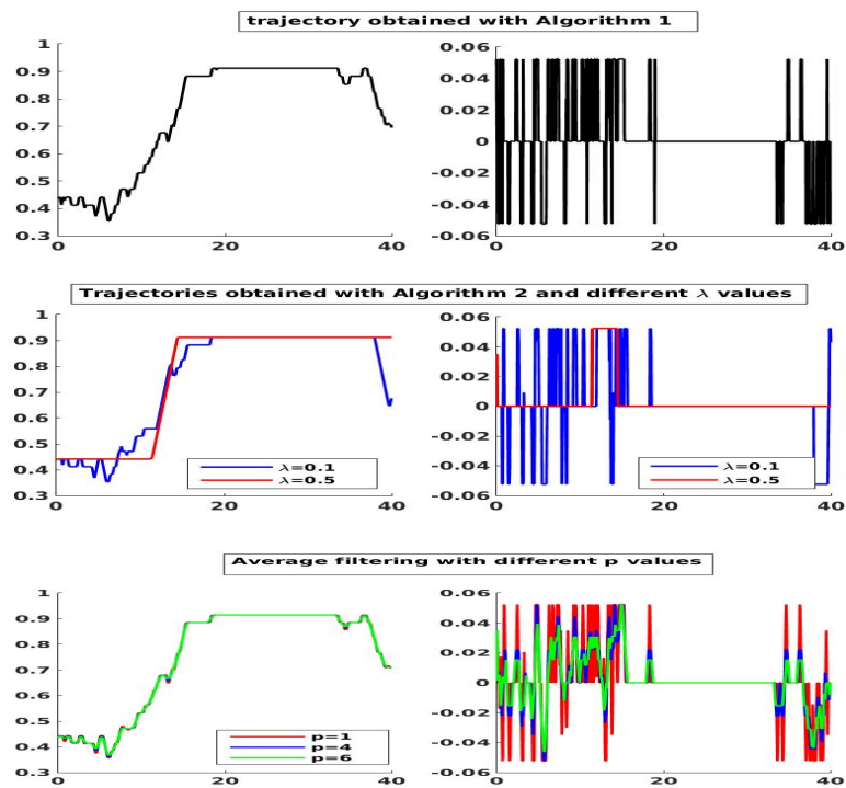
Figure 6: (Test 3) Optimal trajectories (left) and corresponding control u (right), obtained using different reconstruction procedures.
