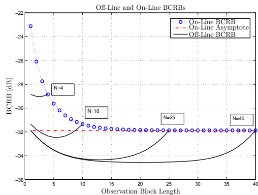
Fig. 4. BCRBs for various positions and different block lengths, SNR=10dB, \sigma_w/T = 10^{-4} , BPSK in DA mode.
