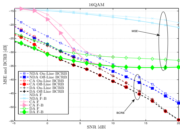
Fig. 8. On-Line and Off-Line BCRB versus SNR, \sigma_w/T = 10^{-4} , Block length = 2000, 16QAM signal.
