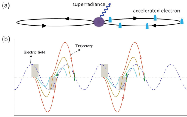
FIG. 4. (a) Schematic illustration of electron recollision excitation. (b) Trajectories of the electrons (solid lines) in the laser field (blue dashed line), which lead to the periodic recollision excitation of the parent ion. The recollision occurs from opposite sides of the parent ions, leading to interference of the dipole moments, with the direction of the recolliding electrons indicated by the arrow (green).
