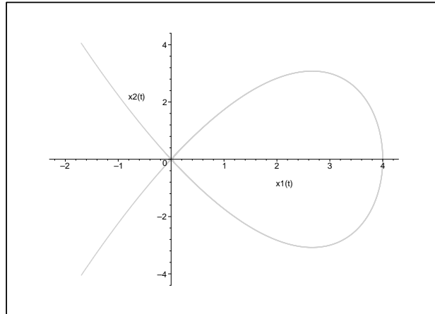
Fig. 5.3. Ensemble \{L(x) = 0\}
