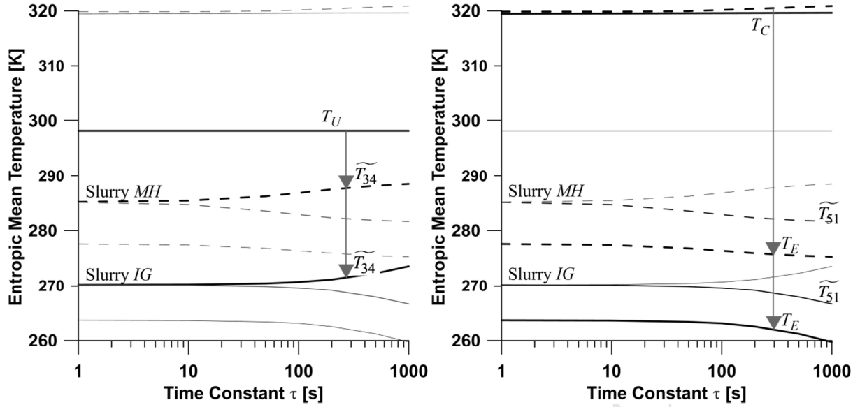
Fig. 6: Entropic mean temperatures \widetilde{T}_{34} and \widetilde{T}_{51} as functions of the kinetics time constant, and interpretation with respect to energy efficiency. Left side: Transfers in HXU are ruled by the temperature difference T_U - \widetilde{T}_{34} , represented by the grey vertical arrows. Right side: total energy consumption is mainly governed by the temperature difference T_C - T_E (grey vertical arrows), with the latter temperature following the variations of \widetilde{T}_{51} .
