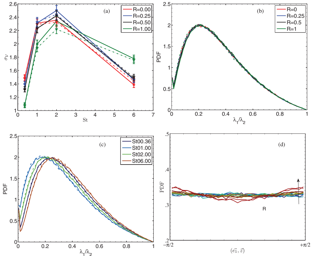
FIG. 4. Voronoï analysis on 2D slices. Standard deviation of the Voronoï areas as a function of St at fixed R (a). PDFs of cell aspect ratio for St = 2 for each R (b) and for R = 0.5 for each St (c). PDFs of the angle between the Voronoï cells' principal axis of inertia \vec{e}_1 and the gravity direction \vec{z} for each (St, R) values (d). When relevant, full line correspond to slices in planes containing gravity and dashed-dotted lines to planes perpendicular to gravity.
