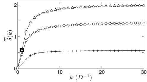
FIG. 8. \tilde{\delta}(k) as function of k for TM73(+) setups without ( \Delta ) and with annulus ( \circ ). The specific data point \tilde{\delta}(1/D) is represented with a large black symbol ( \blacksquare ). The difference \Delta\tilde{\delta}(k) between the two curves is also displayed ( + ). At high k , this difference converges asymptotically to \Delta\tilde{\delta} and is of the order of \tilde{\delta}(1/D) without annulus (see text for details). Wavenumbers are normalized by the PIV window size D=1.93R .
