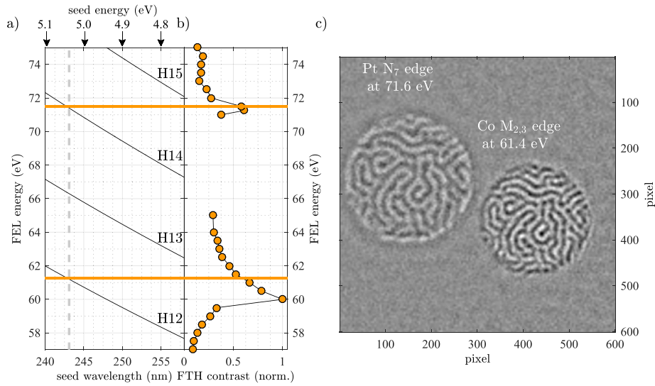
FIG. 6. (a), (b) FEL energy as a function of seed wavelength shown for harmonics H12 to H15. For a single seed wavelength of \lambda_{\text{SEED}} = 242.2 nm, we can maximize the magnetic domain contrast at the Pt N 7 edge at 71.6 eV (H14) and simultaneously get a comparable signal for H12 at 61.4 eV at the Co M 2,3 edge. (c) Element specific magnetic domain patterns for Pt and Co reconstructed from a single difference hologram. The respective element specific real space information for Co and Pt does not overlap. Note that the pixels correspond to different real-space coordinates due to the different XUV wavelengths employed.
