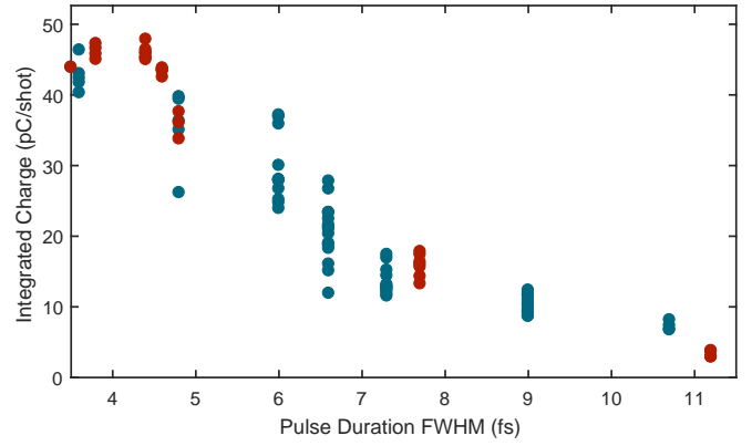
FIG. 3. Total detected charge as a function of pulse duration for a delay \Delta t = 90 ps between the prepulse and the main pulse. The pulse duration is tuned here by chirping positively (red points) or negatively (blue points) the 3.5-fs driving laser.
