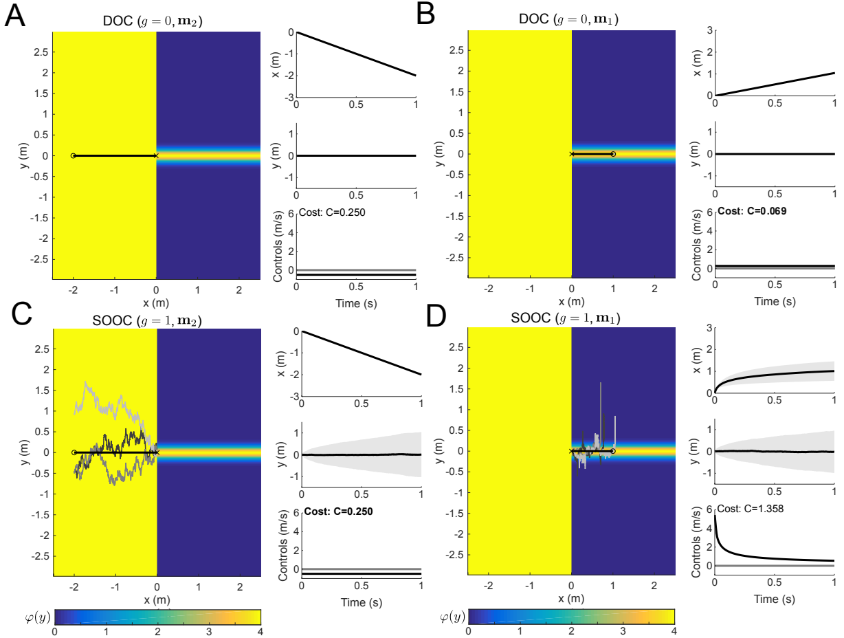
Figure 1. Comparison of DOC and SOOC. A. Deterministic case ( g = 0 ) and final state \mathbf{m}_2 . The colormap illustrates the landscape defined by the function \varphi(y) . The thick black path indicates the optimal mean trajectory. The 3 subplots on the right depict the time evolution of mean positions along the x and y axes, and the optimal open-loop controls (black for u(t) and gray for v(t) ). B. Same information for the deterministic case ( g = 0 ) and final state \mathbf{m}_1 . In the deterministic settings, as the optimal cost to move to \mathbf{m}_1 is smaller than the optimal cost to move to \mathbf{m}_2 , the optimal strategy is thus to use the shortest path (i.e. to move rightward, the optimal cost being emphasized in bold). C. Stochastic case ( g = 1 ) and final state \mathbf{m}_2 . In addition to the colormap and the optimal mean trajectory, here we also display three instances of noisy trajectories to illustrate the stochastic nature of the paths. The 3 subplots on the right depict the same information as before but, here, mean trajectories were estimated from 1 000 samples (depicted in thick traces). Shaded areas depict standard deviations. D. Same information for the stochastic case ( g = 1 ) and final state \mathbf{m}_1 . Here, we see that the optimal strategy is to reach to the left target because the cost is smaller (emphasized in bold). This is because, in the right part of the plane ( x \geq 0 ), the controller has to steer quickly the system to the target before it is shifted away from the midline, toward locations where it will be more difficult (i.e. energy consuming) to move. Parameters were as follows: c = 4 , \sigma = 0.01 and T = 1 .
