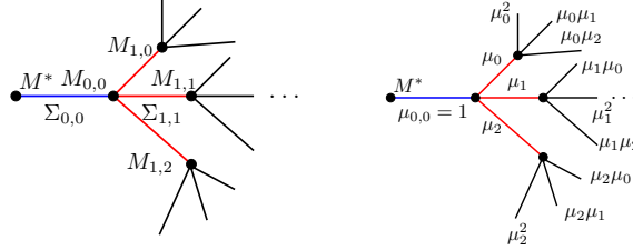
Fig. 1 A self-similar 3-adic infinite tree. Left: In blue we mark the edges that belong to \mathcal{G}^0 , in red the edges of \mathcal{G}^1 , in black the edges of \mathcal{G}^2 . Right: Distribution of weights on the edges of a 3-adic infinite self-similar tree.
