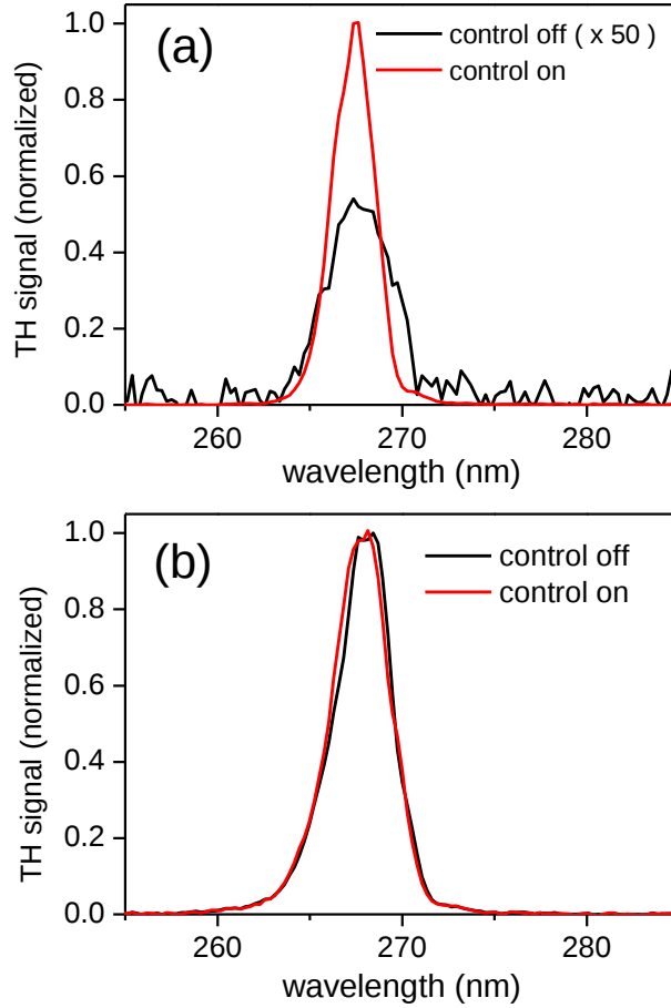
Fig. 5. Effect of crossing filament on the TH generation. The focal lens for (a) and (b) are 1000 mm and 200 mm respectively. The focal length for the control pulse was 500 mm and the control pulse energy was 380 \mu J, similar to that in ref [24].
