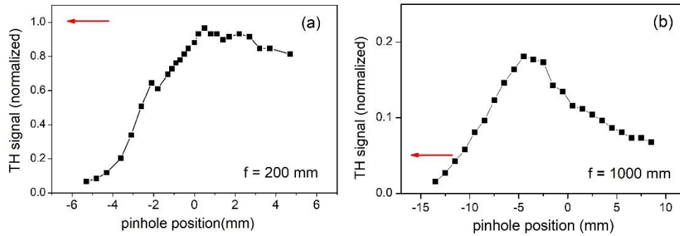
Fig. 2. The third harmonic signal pass through a 110 \mu m pinhole scanned along the filament. (a) f = 200 mm. (b) f = 1000 mm. The origin ( z = 0 mm) is defined as the geometrical focus in each cases.
