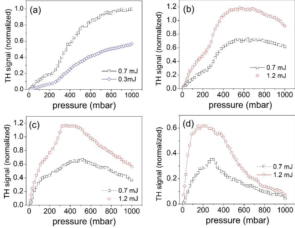
Fig. 3. Third harmonic signal as a function of air pressure for different focal lengths. From (a) to (d), the focal lengths are 200 mm, 500 mm, 750 mm, and 1000 mm respectively. All the data are normalized to the signal obtained with 0.7 mJ incident pulse energy in the case of f = 200 mm and 1 bar air.
