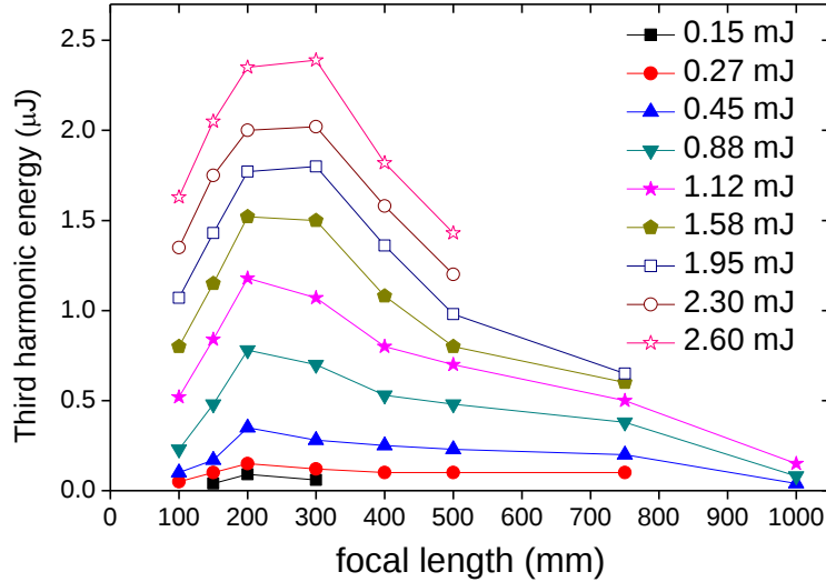
Fig. 1. Third harmonic yield as a function of focusing length for different incident pulse energies. The diameter of the incident pulse is 14 mm.
