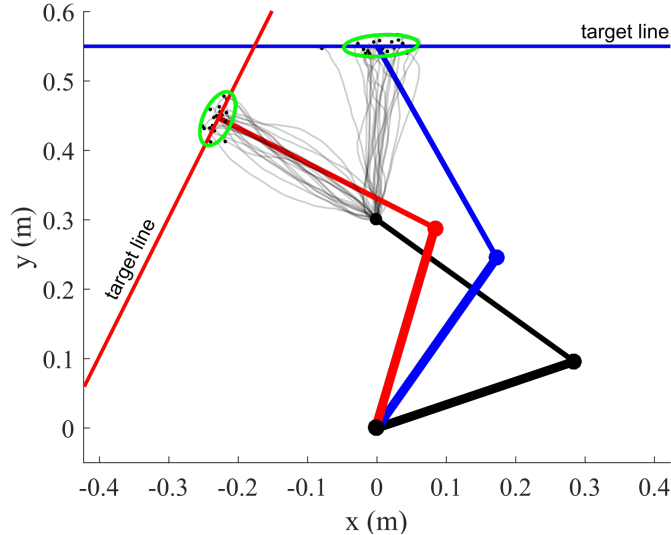
Figure 6. Top view of arm trajectories for a pointing-to-a-line experiment. The targets are indicated by the solid lines (blue and red). The green ellipse represents the 90% confidence ellipse of the endpoint distribution. Noise was additive ( \sigma_i = 0.1 ) in these simulations and movement time was t_f = 0.75 s for the forward motion (blue) and t_f = 0.55 s for the leftward motion (red). The variance weight in the cost, q_{var} , was set to 10^4 and endpoint variance was penalized in the direction orthogonal to the target line (via the function \mathbf{n}^\top J(\mathbf{q}_f) P_{\mathbf{q},f} J(\mathbf{q}_f)^\top \mathbf{n} where \mathbf{n} is the normal vector, J is the Jacobian matrix and P_{\mathbf{q},f} is the joint-space positional covariance). Note that hard terminal constraints were imposed on the mean state (mean endpoint position on the target line and zero final mean velocity). The main orientation of the endpoint confidence ellipses is compatible with experimental observations and shows that co-contraction may be used to increase accuracy in the task-relevant dimension.
