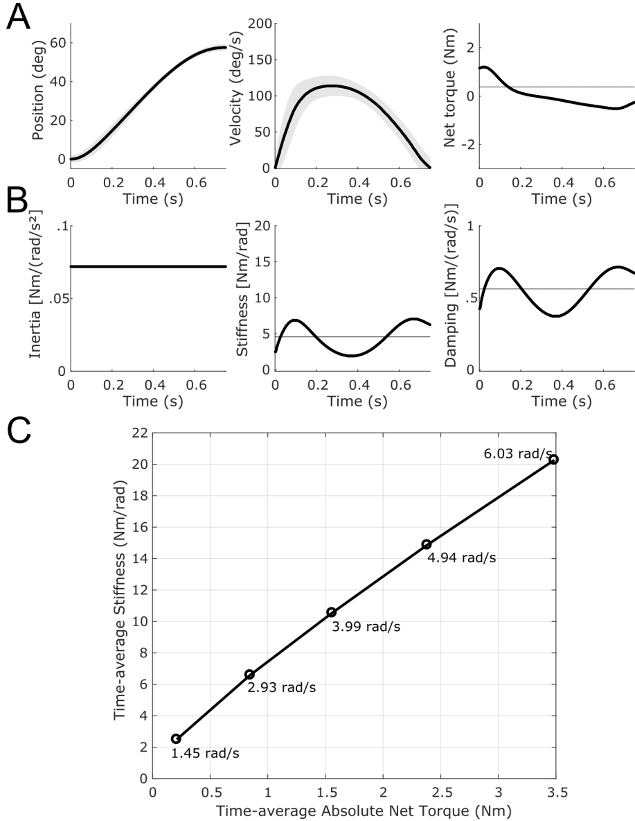
Figure 2. Simulations of a forearm pointing movement (elbow extension of 1 rad). A. Optimal trajectories. Angular displacement and velocity profiles (mean in thick lines and standard deviation in shaded areas) and net torque responsible of the joint motion (third column). B. Optimal impedance. Inertia (constant for this single-joint system), stiffness and damping are depicted. Time-varying joint stiffness and damping, part of the open-loop optimal motor plan in our model, are responsible of robustness of motor behavior around the mean behavior (without needing on-line feedback for that purpose). Note an increase of stiffness at the end of the motion, to improve accuracy on target, in agreement with experimental data. Values can be quantitatively compared to [59]. Time-average values are represented by horizontal lines. C. Relationship between time-average net torques and time-average stiffnesses for movements of different speeds. Peak velocity is indicated in rad/s. An approximately linear relationship is observed as in [54]. In panels A and B, parameters were as follows: q_{var} = 10^4 , \alpha = 1 , \beta = 0.01 , t_f = 0.75 , and I = 0.072 . In panel C, parameters were the same except that q_{var} = 5 \times 10^3 and t_f ranged between 0.25 s and 1.0 s to generate movements of different speeds.
