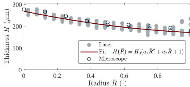
Figure 7: Measured thickness of the membrane as a function of the non-dimensional radius. The fitting parameters are H_0 = 268 \mu\text{m} , a_1 = 0.23 , and a_2 = -0.59 .
