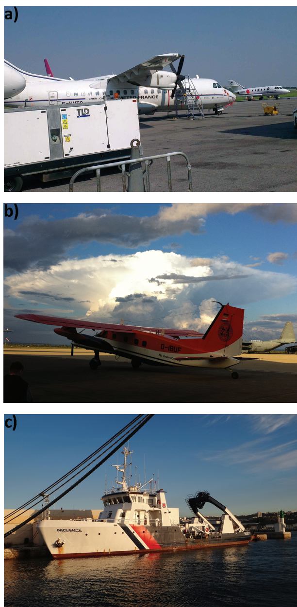
FIG. 7. (a) French and (b) German aircraft deployed during SOP1, (c) Le Provence operated during SOP2, and (d) pressurized boundary layer balloons launched from Candillargues during SOP2. The French ATR42 (foreground) and Falcon 20 (background) in (a) were based at Montpellier airport and the German Dol28 in (b) was based in Corsica at Solenzara airport. [Source: (a),(d): P. Drobinski; (b) C. Kottmeier; (c) I. Taupier-Letage.]
