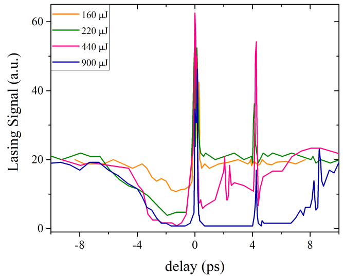
Fig. 2. Time-integrated lasing signal obtained with consecutive pump and control pulses. Pump pulse has 1.1 mJ energy, control pulse energy is indicated in the legend, N_A=0.01 . N_2 gas pressure is 100 mbar.
