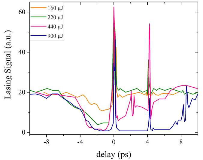
Fig. 2. Time-integrated lasing signal obtained with consecutive pump and control pulses. Pump pulse has 1.1 mJ energy, control pulse energy is indicated in the legend, N_A=0.01 . N_2 gas pressure is 100 mbar.
