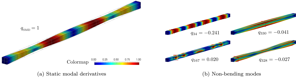
Fig. 5: (a) Static modal derivative \boldsymbol{\theta}_{11} associated to the first bending mode. (b) Four first non-bending modes contained in the SMD \boldsymbol{\theta}_{11} , found equivalently by projecting \boldsymbol{\theta}_{11} on the linear mode basis, or by application of Eq. (23). The relative modal participation factors q_s of each of these modes numbered 34, 167, 328 and 330 (see also Table 1) is also numerically given, normalized by the total amplitude of the SMD \boldsymbol{\theta}_{11} ( q_{SMD} = 1 ), and exactly recovers the factors exhibited in Eq. (23).
