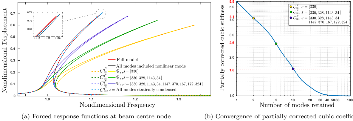
Fig. 4: Convergence to the full model solution with the increase of coupled modes taken into account in the reduced model. (a) Frequency response curve of the beam at center, in the vicinity of the first bending mode eigenfrequency; case of the thick beam with 1287 dofs. Red: full model, and convergence curves with increasing number of modes retained in the truncation: 1 mode (yellow), 4 modes (green), 9 modes (blue), all modes statically condensed (dashed light blue). Solution with one NNM in black. (b) Convergence of the evaluated corrected cubic stiffness coefficient T_{111}^1 , defined in Eq. (16), with increasing number of linear modes kept in the truncation.
