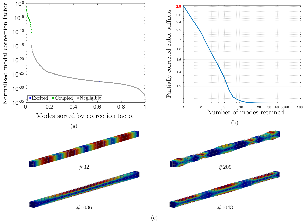
Fig. 8: Convergence without Poisson effect ( \nu = 0 ) for the thick beam. (a) Nondimensional correction factor C_{111}^{1s}/\beta_{111}^1 of all the modes over the nondimensional mode number s/N . (b) Convergence of the evaluated corrected cubic stiffness coefficient \Gamma_{111}^1 , defined in Eq. (16), with increasing number of linear modes kept in the truncation. (c) Mode shapes and order of appearance in the basis (#) of four of the most relevant modes coupled with the first bending mode.
