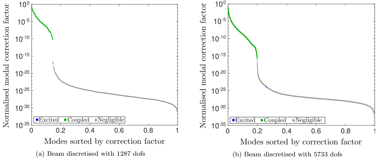
Fig. 3: Nondimensional correction factor C_{111}^{1s}/\beta_{111}^1 (Eq. (17)), associated to the first bending mode ( p = 1 ) and to all the other modes ( s = 2, \dots, N ) of the thick beam testcase, over the sorted nondimensional mode number s/N , where the imposed order is by decreasing correction factor. The Poisson ratio is \nu = 0.3 .
