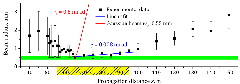
Figure 4. The dependence of the average beam radius on the distance z (squares) and its linear fit in the range z = 65\text{--}95 m (blue line). The green horizontal band shows the minimum value of the radius. Yellow rectangle is the range z = 55\text{--}95 m, where the beam propagates in postfilamentation regime. Radius of Gaussian beam at e^{-1} with waist w_0 = 0.55 mm (red line) vs. z .
