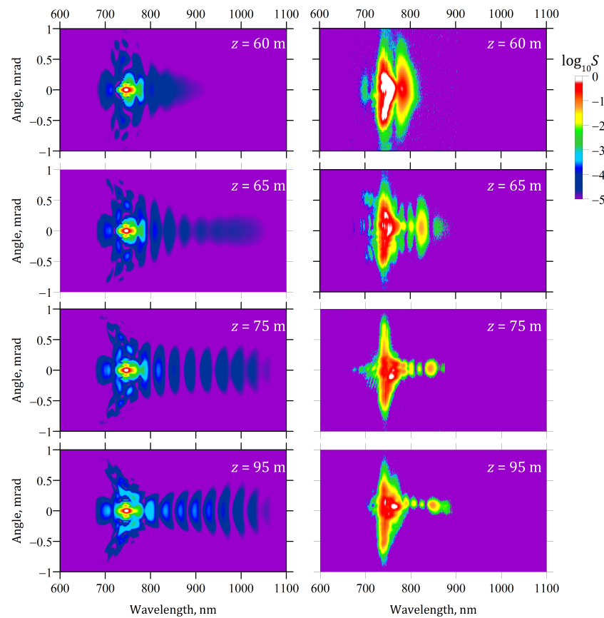
Figure 5. The angle-wavelength spectra obtained in numerical simulations (left column) and in the experiment (right column) at the distances from 60 m to 95 m.
