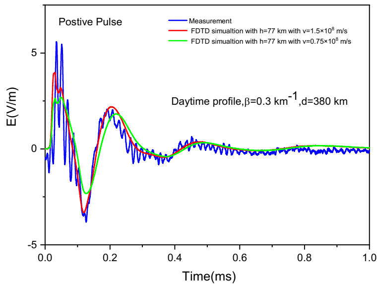
Fig. 10. Comparison between the FDTD simulation and experimental data for the positive pulse (Positive RS in Fig. 3a) of the bipolar flash of 21 September 2014, 15:14:09 (local time) considering the return-stroke speed 1.5 \times 10^8 m/s (red line) and 0.75 \times 10^8 m/s (green line). h = 77 km and \beta = 0.3 km -1 were adjustable parameters that were varied to achieve the best match to the measured waveform.
