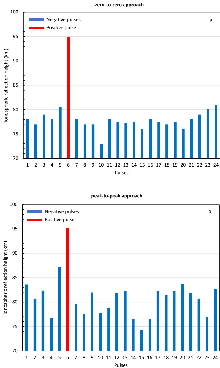
Fig. 7. Sequence of evaluated reflection heights for 23 negative and one positive pulses of the flash of 21 September 2014, 15:14:09 (local time) using a) zero-to-zero approach and b) peak-to-peak approach.
