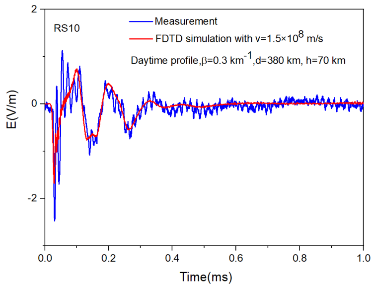
Fig. 11. Comparison between the FDTD simulation and experimental data for the negative return stroke labeled RS10 (in Fig. 3a) of the bipolar flash of 21 September 2014, 15:14:09 (local time).
