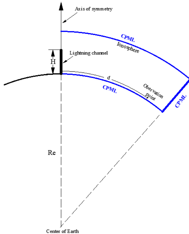
Fig. 9. The geometry of the FDTD model.
