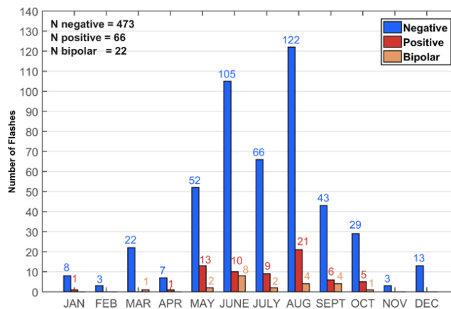
Fig. 1. Monthly distribution of negative, positive and bipolar lightning flashes recorded at Sântis Tower over the period ranging from June 2010 to July 2016.
