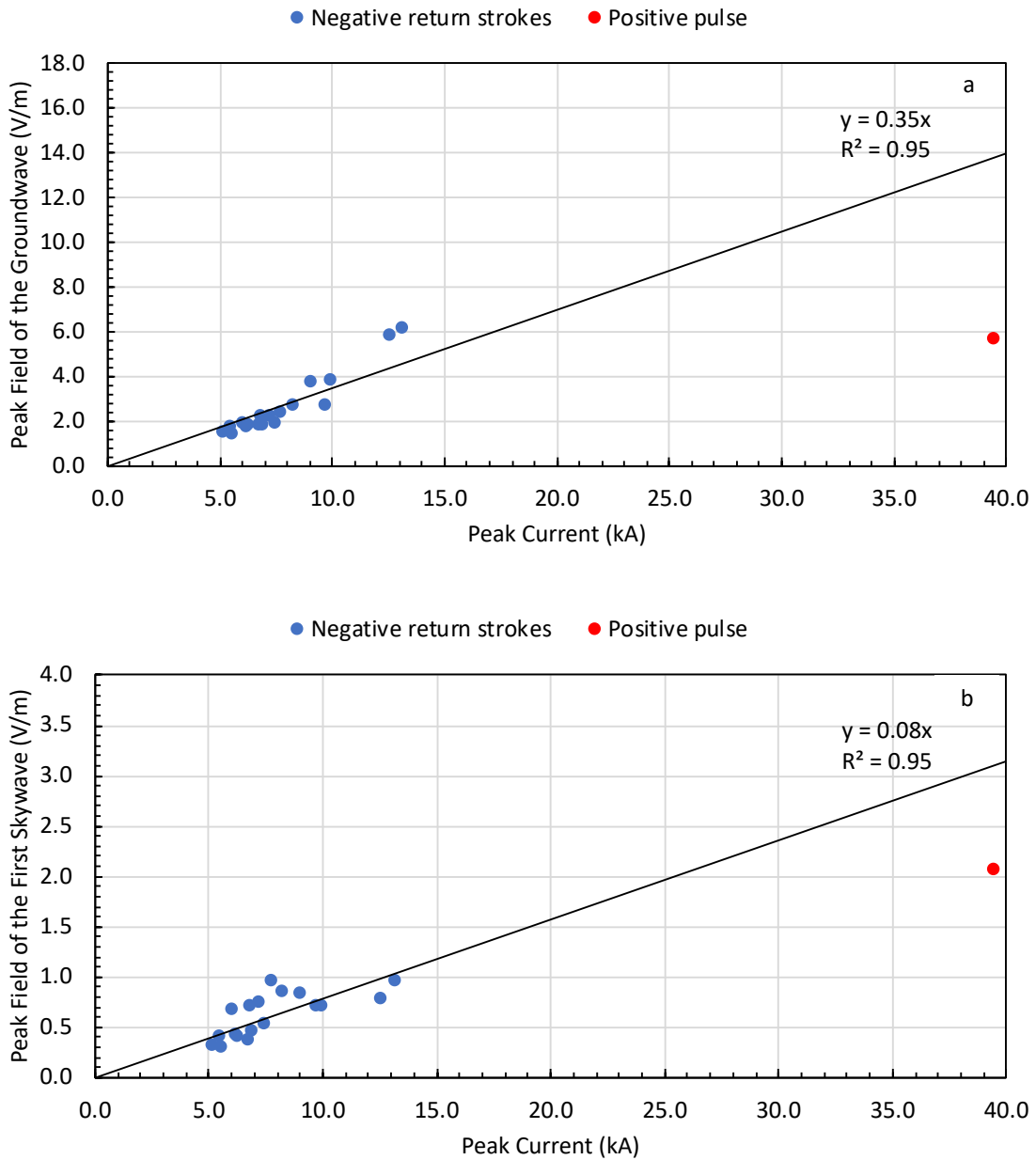
Fig. 8. Electric-field peak of a) the groundwave and b) the first skywave at 380 km versus current peak for all the pulses of the flash of 21 September 2014, 15:14:09 (local time). The positive pulse is shown in red and the 18 negative pulses are shown in blue. The best fit linear regression for negative return strokes is also shown in the figure.
