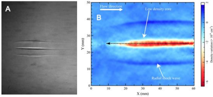
Figure 1.7 Image a low-density channel observed 6 \mu\text{s} after the filament formation in air. A) Schlieren image showing the radial shockwave. B) Density map obtained by interferometry [17].
