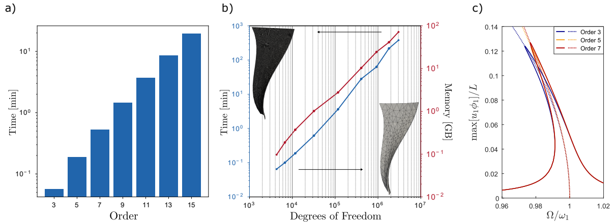
Fig. 12 (a) Computing times required to reach a given parametrisation order, for the 11727 degrees of freedom mesh. (b) Computing times required to perform an order 5 parametrisation with RNF style, for meshes of increasing refinement. (c) Convergence of the forced response curve and backbone with the order, for the 3 millions degrees of freedom mesh. All the analyses were performed on a desktop workstation with an AMD®Ryzen 5950X processor at 4.9 GHz and 128GB RAM.
