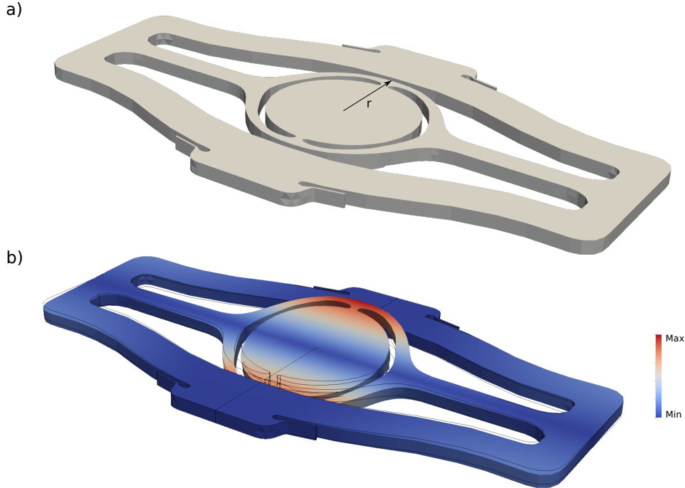
Fig. 10 (a) MEMS micromirror geometry. (b) Magnified displacement field associated to the third eigenmode of the structure.
