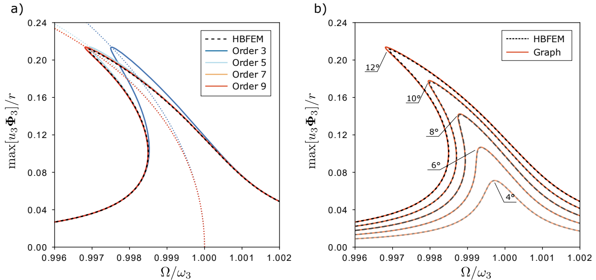
Fig. 11 Frequency-response functions for the MEMs micromirror. The modal displacement u_3 is normalised by the maximum of the third eigenvector \Phi_3 and the radius r ; the nonlinear frequency \omega is normalised by the linear frequency \omega_3 of the third mode. (a) Convergence of a graph style parametrisation by varying the expansion order for \kappa = 3 \mu\text{m}/\mu\text{s}^2 and comparison with reference HBFEM. (b) Comparison between HBFEM solution and order 9 expansion for load multiplier \kappa values equal to 1.0, 1.5, 2.0, 2.5, and 3.0 \mu\text{m}/\mu\text{s}^2 . Tags report the physical rotation angle reached by the device at the peak of the FRF.
