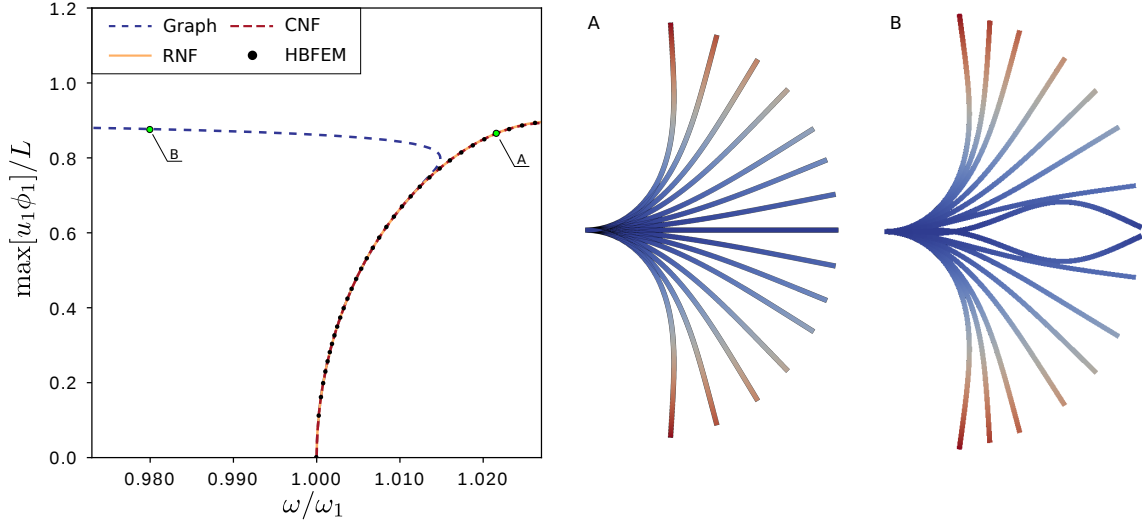
Fig. 7 Backbone curve of fundamental mode of the cantilever beam. Comparison between full-order model solution (reference) computed with an HBFEM method (black points) and ROMs up to order 25 (converged solution) for graph (dotted blue), RNF and CNF (orange and dashed red) styles. The modal displacement u_1 is normalised by the maximum of the first eigenvector \Phi_1 (equivalent to the first master eigenvector \phi_1 ) and the length L ; the nonlinear frequency \omega is normalised by the linear frequency \omega_1 of the first mode. Panels A and B show snapshots of the deformation field of the structure at points A and B shown in the left (A: normal form style, B: graph style).
