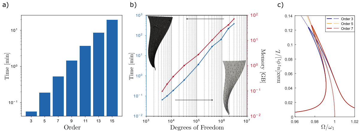
Fig. 12 (a) Computing times required to reach a given parametrization order, for the 11727 degrees of freedom mesh. (b) Computing times required to perform an order 5 parametrization with RNF style, for meshes of increasing refinement. (c) Convergence of the forced response curve and backbone with the order, for the 3 millions degrees of freedom mesh. All the analyses were performed on a desktop workstation with an AMD®Ryzen 5950X processor at 4.9 GHz and 128GB RAM.
