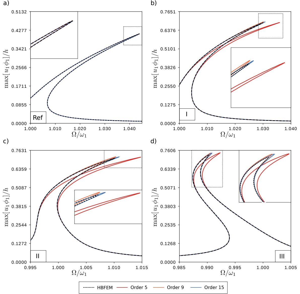
Fig. 4 Frequency-response curves for the arched structures. Comparison between full-order HBFEM simulations and ROMs obtained from RNF style parametrisation. (a) Reference flat beam, (b) Arch I. (c) Arch II. (d) Arch III. The modal displacement u_1 is normalised by the maximum of the first eigenvector \Phi_1 (equivalent to the first master eigenvector \phi_1 ) and the thickness h ; the forcing frequency \Omega is normalised by the linear frequency \omega_1 of the first mode.
