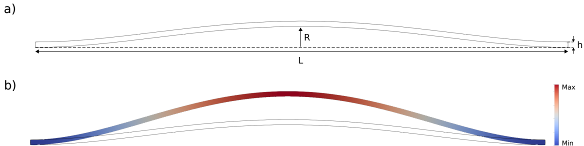
Fig. 2 (a) Schematic representation of the shallow arch geometry, with thickness h = 6.4 \mu\text{m} , and length L = 640 \mu\text{m} . The rise of the arch R for the three configurations is R_I = 2.40 \mu\text{m} , R_{II} = 2.88 \mu\text{m} , R_{III} = 3.36 \mu\text{m} . The out-of-plane thickness of the arch is 32 \mu\text{m} for all geometries. (b) Magnified displacement field associated to the first eigenmode of the structure.
