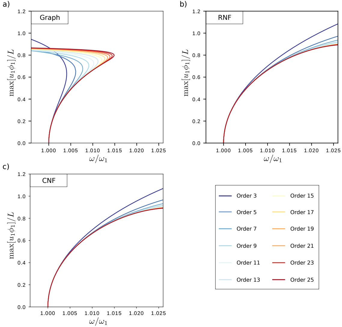
Fig. 6 Backbone curves of the fundamental mode of the cantilever beam. Convergence of the asymptotic expansion upon a change in order for different parametrisations: (a) graph style, (b) RNF style, and (c) CNF style. Data are reported for expansions from order 3 to order 25. The modal displacement u_1 is normalised by the maximum of the first eigenvector \Phi_1 (equivalent to the first master eigenvector \phi_1 ) and the length L ; the nonlinear frequency \omega is normalised by the linear frequency \omega_1 of the first mode.
