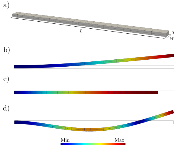
Fig. 3 (a) Cantilever geometry. The structure has a length L equal to 1 m, a width W equal to 0.05 m, and a thickness T equal to 0.02 m. Pictures (b), (c), and (d) depict the displacement fields associated to the first bending mode \Phi_{B_1} , the first axial mode \Phi_{A_1} (which is mode number 10 in the order of increasing frequencies for this specific beam), and the second bending mode \Phi_{B_2} , respectively. Displacement magnitude is scaled to improve the readability of the images.
