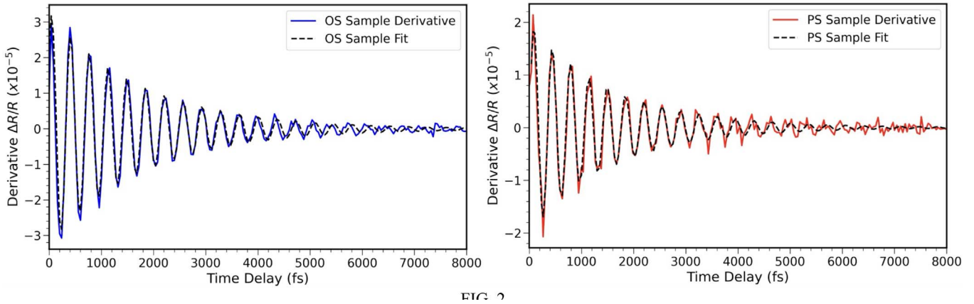
Fig. 2. Derivative of the experimental results with fitted curves for both OS (left panel) and PS (right panel) samples.
