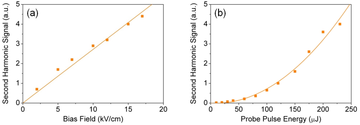
Figure A.8: Measured second harmonic signal as a function of biased field (a) and probe pulse energy (b). For the measurement in (a) the probe pulse energy was 200 \mu J. The bias field was 15 kV/cm for the measurement in (b).
